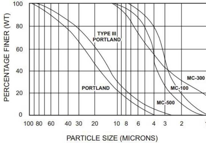
DeNeef Micro Fine Cement Chart
